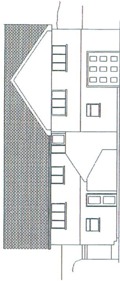
East Elevation
